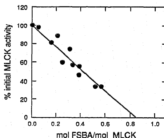
Fig. 4. Stoichiometry of [ ^{14}\text{C} ]FSBA incorporation into skMLCK. Samples of skMLCK were incubated with [adenine-8- ^{14}\text{C} ]FSBA, 0.8 mM, for varying periods of time, then analyzed for remaining enzyme activity and incorporation of [ ^{14}\text{C} ]radioactivity as described in Materials and Methods. Shown plotted is the proportion of enzyme activity remaining versus the mol of [ ^{14}\text{C} ]FSBA incorporated per mol of skMLCK. The line represents a least-squares fit of the data.
