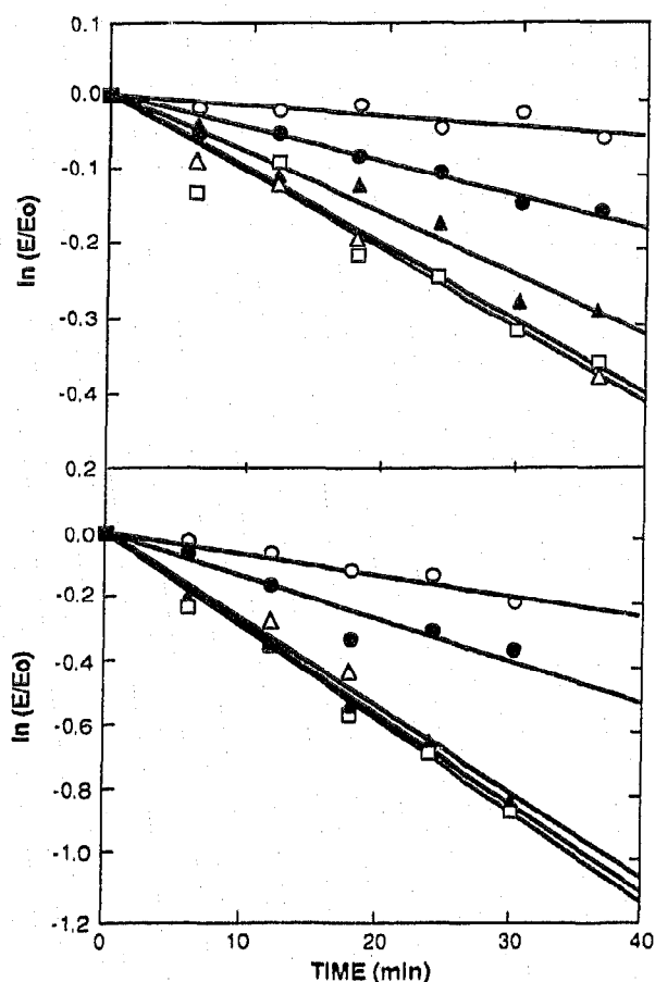
Fig. 3. Inhibition of FSBA inactivation by MgATP. skMLCK [top] or skMLCK · CaM [bottom] was incubated with 0.6 or 0.4 mM FSBA, respectively, under standard conditions with the following modifications. Included in each reaction mixture were either no additional compounds (○), 10 mM MgATP (●), 10 mM MgGTP (△) or 0.2 mM substrate peptide - KKRAARATSNVFA (▲). The open circles (○) represent the average of control values obtained for reaction mixtures containing each of the above-listed compounds, but no FSBA. Average values were presented for the sake of clarity.
