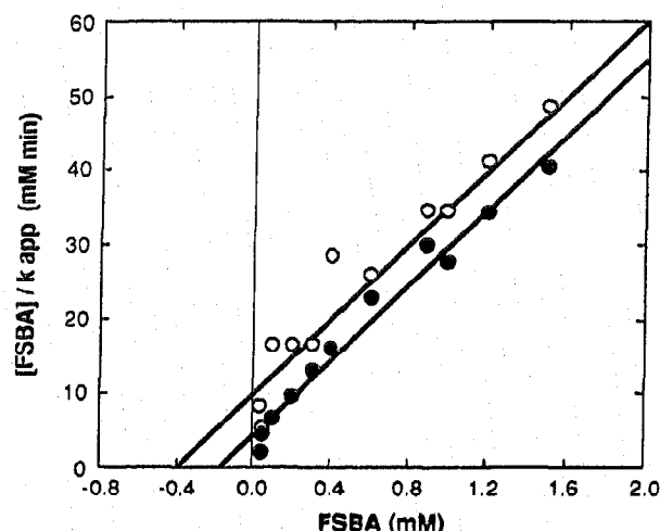
Fig. 5. Analysis of the kinetic parameters for the FSBA inactivation of skMLCK or skMLCK · CaM. Shown is a Hanes-Woolf plot [ S/V versus S ] of the data in Fig. 2 describing the dependence of the rate of inactivation of skMLCK (○) or skMLCK · CaM (●) on the concentration of FSBA. The lines shown represent least-squares fits of the data.
