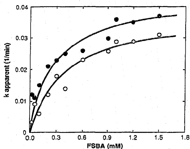
Fig. 2. Dependence of rate of inactivation on FSBA concentration. skMLCK (○) or skMLCK · CaM (●) was incubated with the indicated concentrations of FSBA under standard conditions as described in Materials and Methods. Shown plotted is the apparent first-order rate constant for inactivation, k_{app} , as a function of FSBA concentration.
